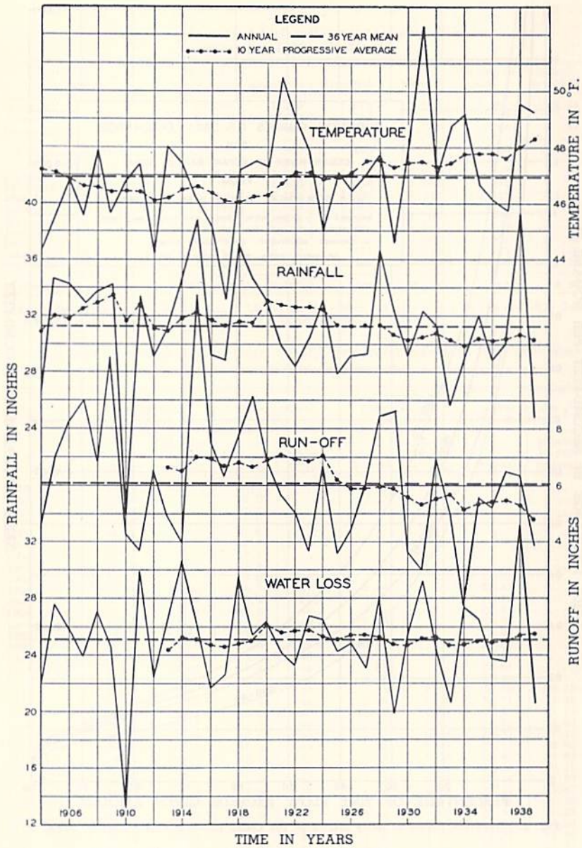
Fig. 3.—Graphs of climatological and runoff data, Cedar River at Cedar Rapids, Iowa.
