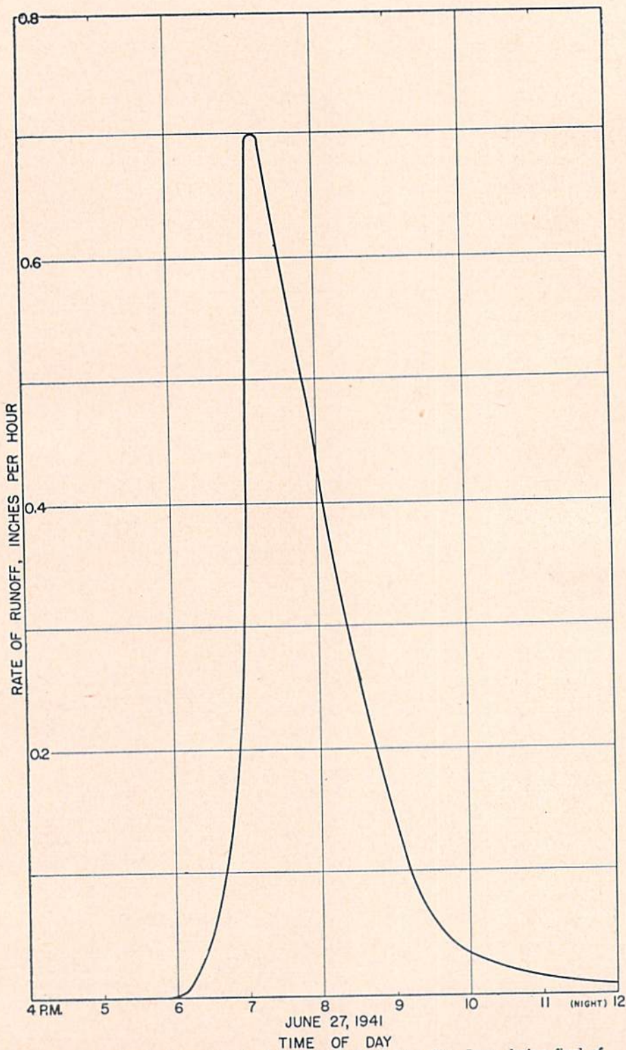
Figure 8.—Graph of runoff rate of Raiston Creek at Iowa City, Iowa, during flood of June 1941.
