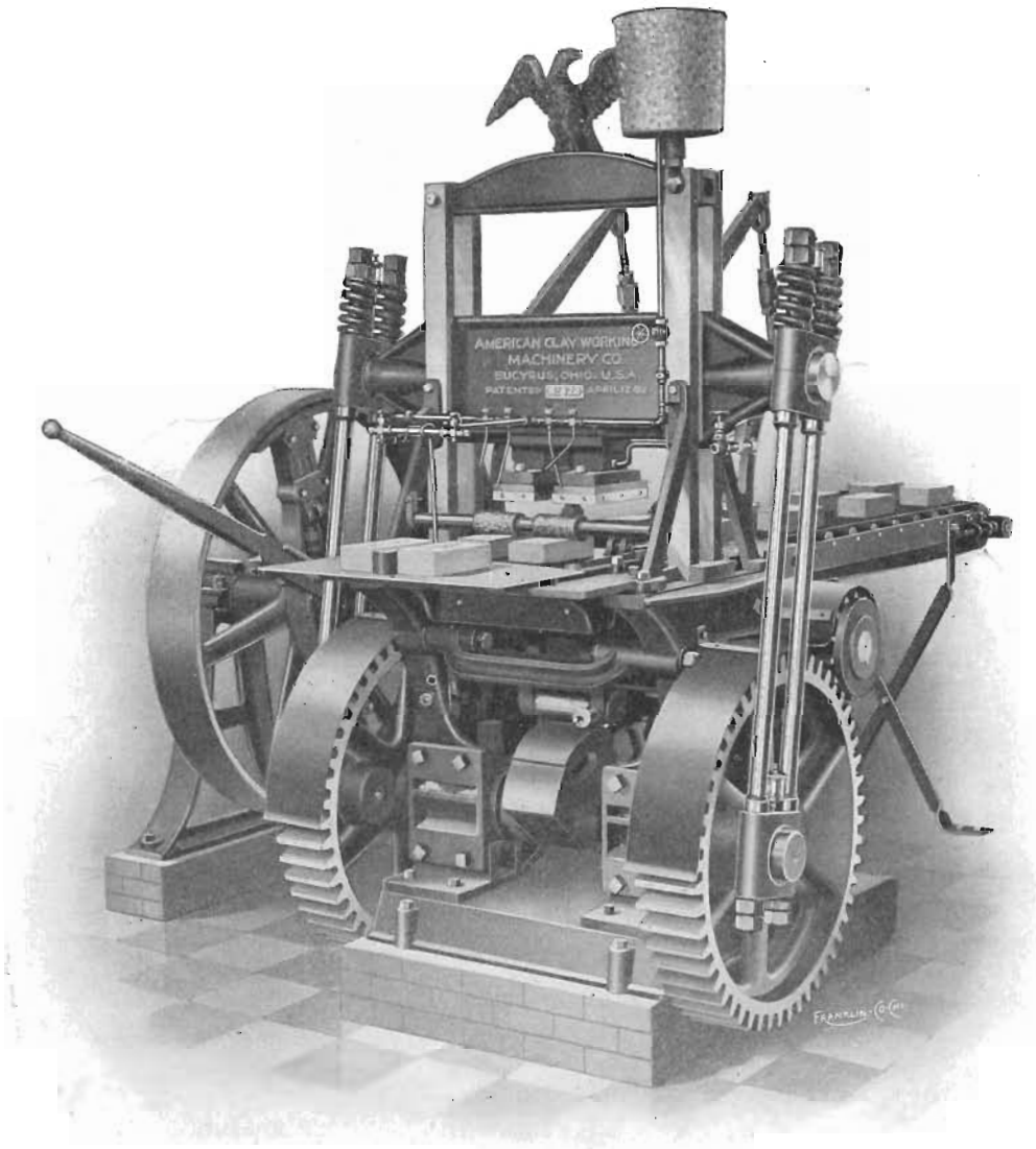
PLATE X. The Eagle Double Die Brick Re-Press. Front View.
