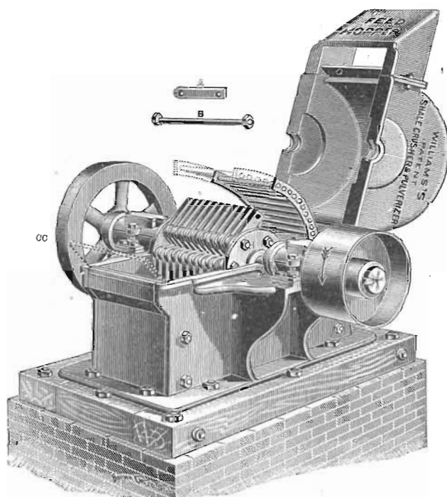
FIG. 11. Williams' Disintegrator and Pulverizer.
