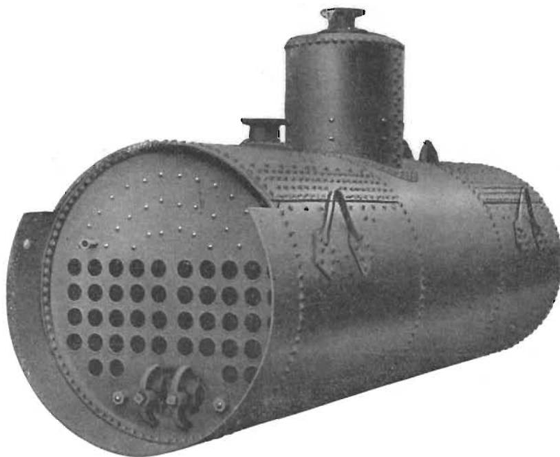
FIG. 31. Boiler with dome, shell extended for full front, wrought iron hinges.
