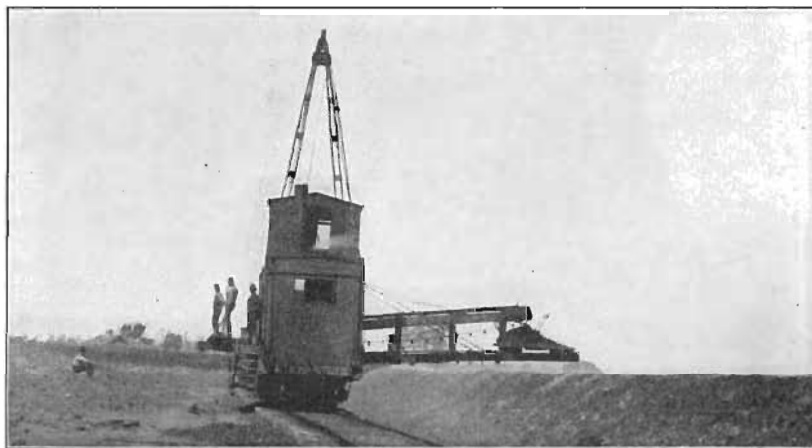
FIG. 77. Coaling machine used by the Davy Burnt Clay Ballast Company.
