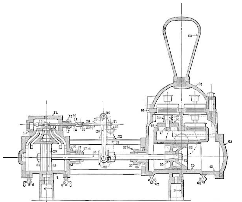
FIG. 35. Duplex pump in section.
