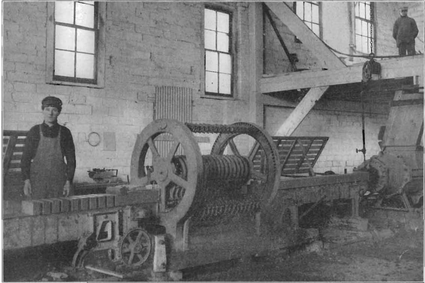
PLATE XXV. A modern rotary cutting table used by the Iowa Brick Company, Des Moines, Iowa.
