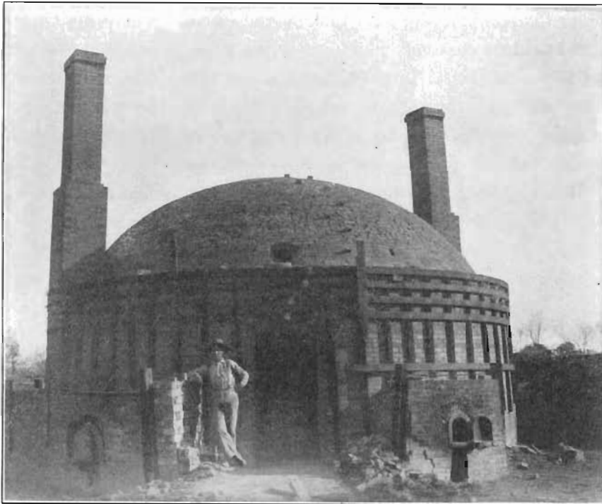
FIG. 28. Round down draft kiln with two stacks.
