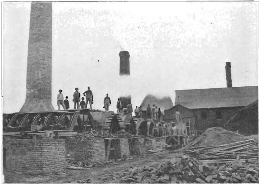
FIG. 62. Modified Dunn continuous kiln in process of construction; Ottumwa Brick and Construction Company, Ottumwa, Iowa.
