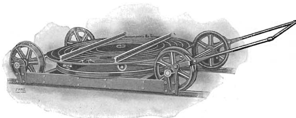
FIG. 26. Combination transfer car and turntable.
