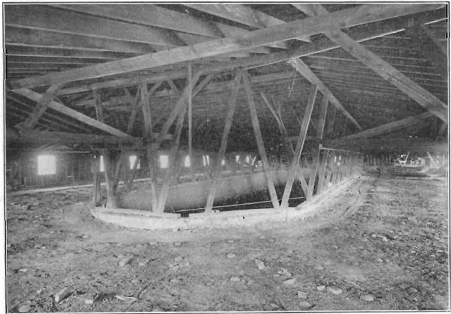
FIG. 73. Top view of Haigh continuous kiln showing arrangement of fire holes and open court.
