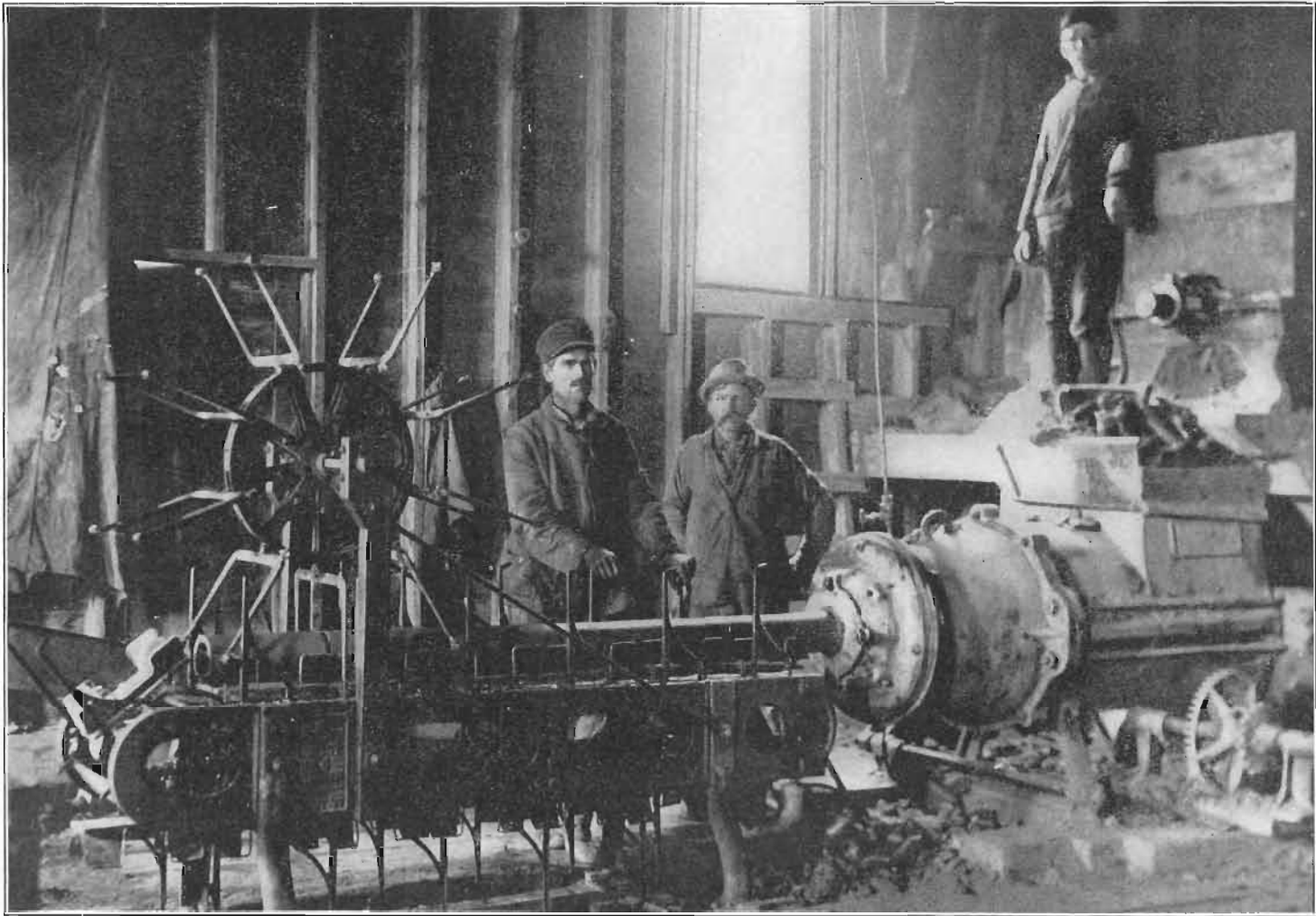
PLATE XXX. Reel cutting table for hollow ware, Lehigh Brick and Tile Company, Lehigh, Iowa.
