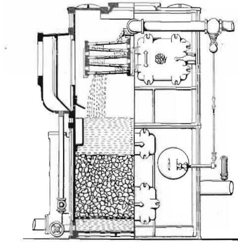
FIG. 39. Sectional view of open feed-water heater.
