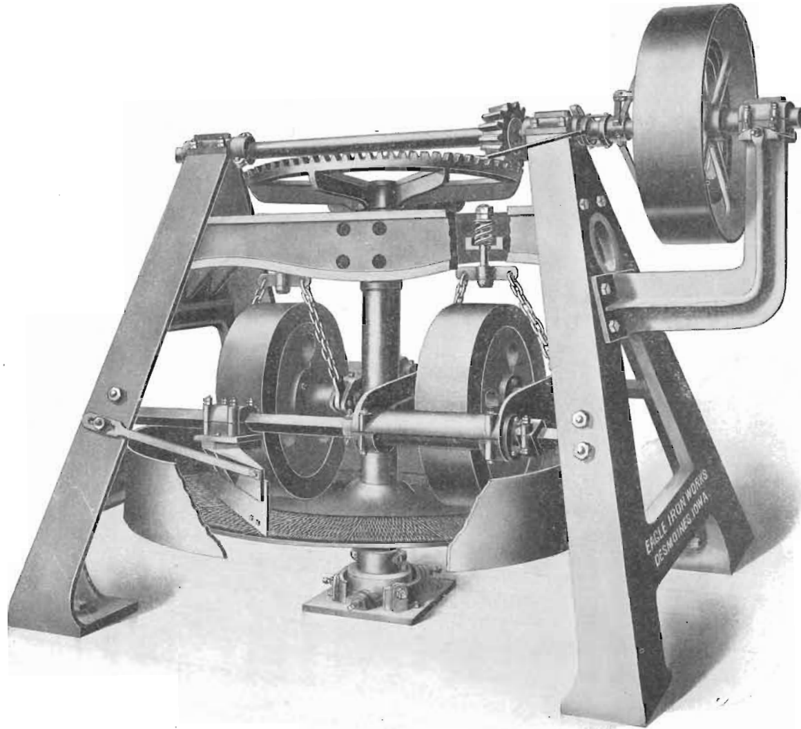
PLATE IV. Standard nine-foot Dry Pan with Steel Frame and Up-to-date Improvements.
