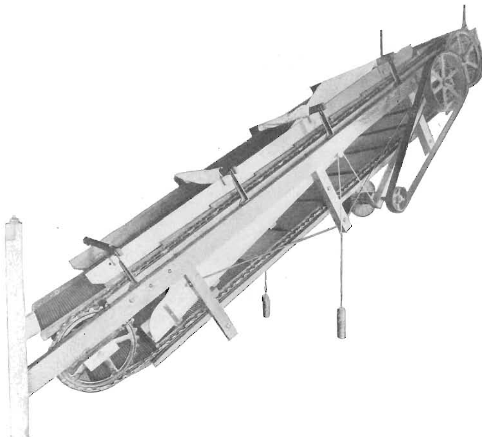
FIG. 13. Type of Revolving Clay Screen with Automatic Brush Cleaner.
