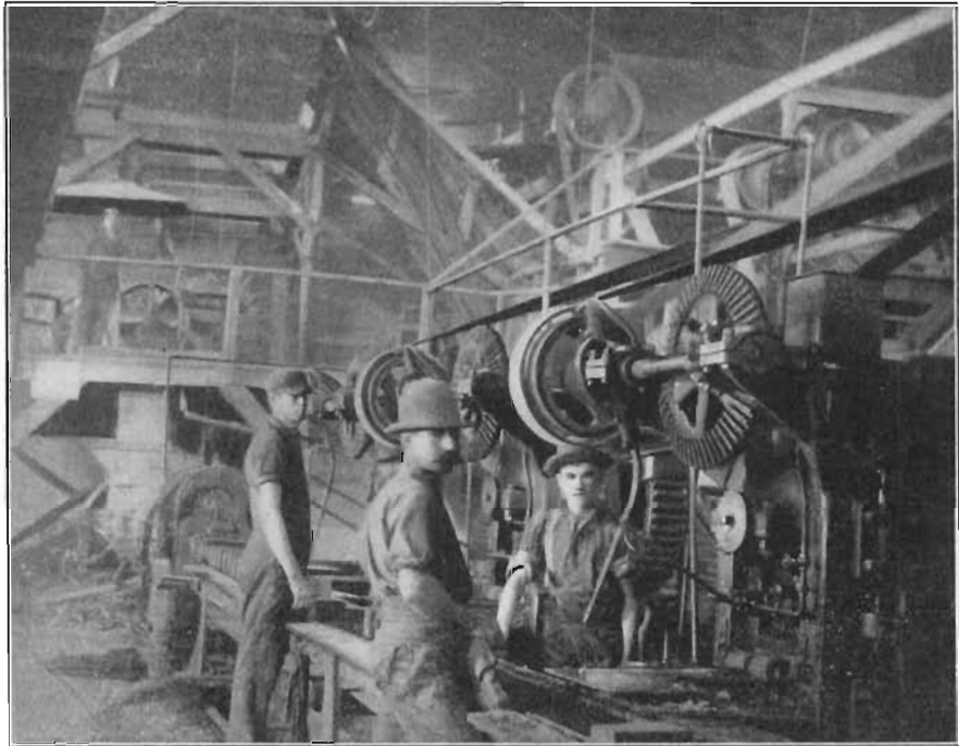
FIG. 54. Represses used by the old Iowa Brick plant, Des Moines, Iowa.
