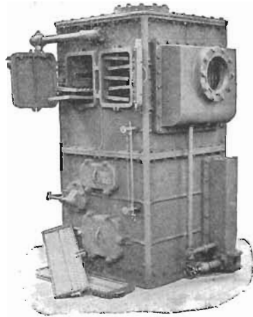
FIG. 38. Type of open feed-water heater.
