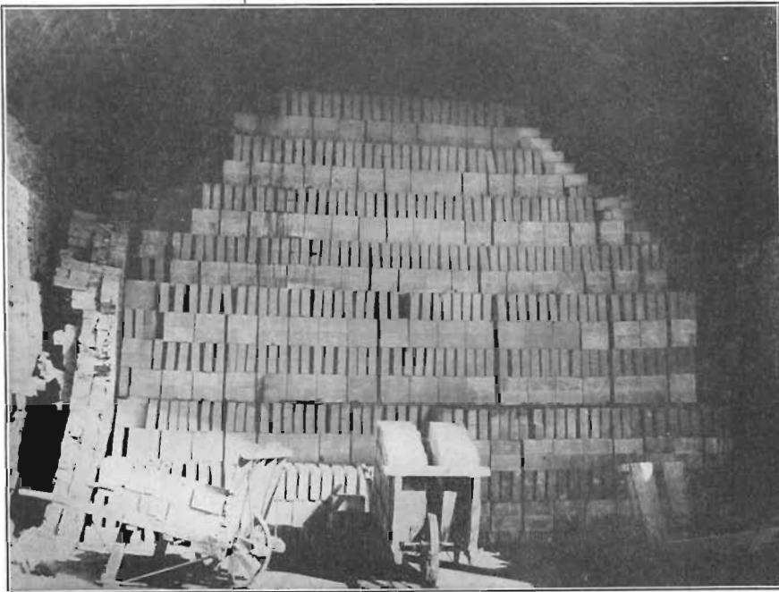
FIG. 30. Interior of rectangular down draft kiln showing method of facing dry pressed brick and a dissected flash wall.
