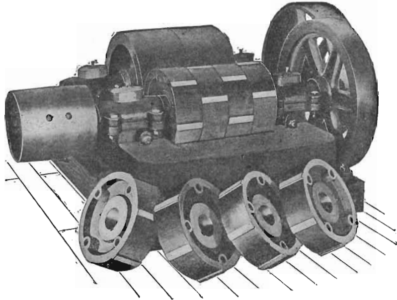
FIG. 8. Clay Crusher, Corrugated Rolls Type.
