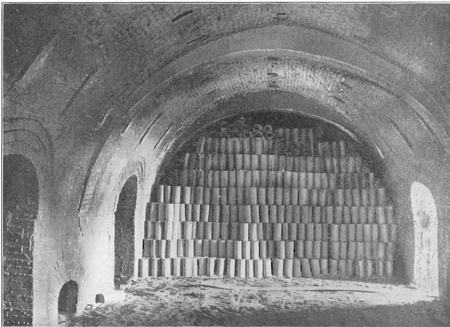
PLATE XXXV. Interior view of Haigh continuous kiln showing method of setting hollow ware. Sioux City Brick and Tile Company, Sioux City, Iowa
