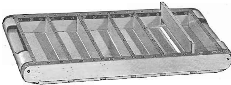
FIG. 15. Common Brick Mold for Soft Mud Brick.
