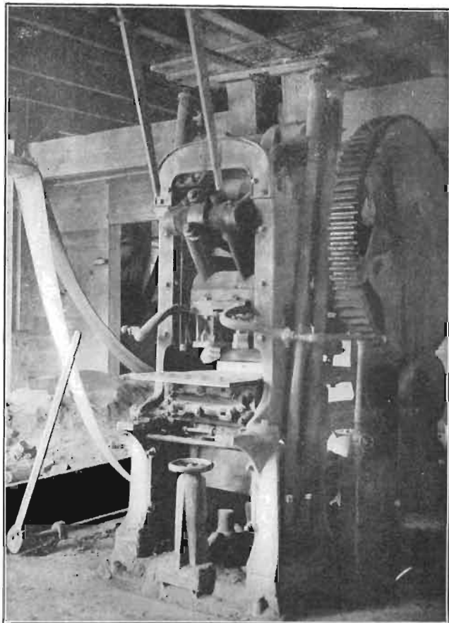
Dry press, shape machine.
