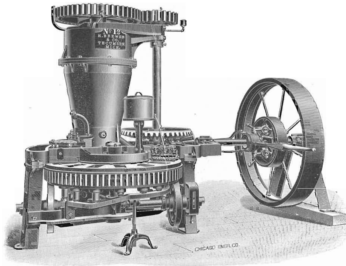
PLATE VI. Vertical Type of Mold Brick Machine.
