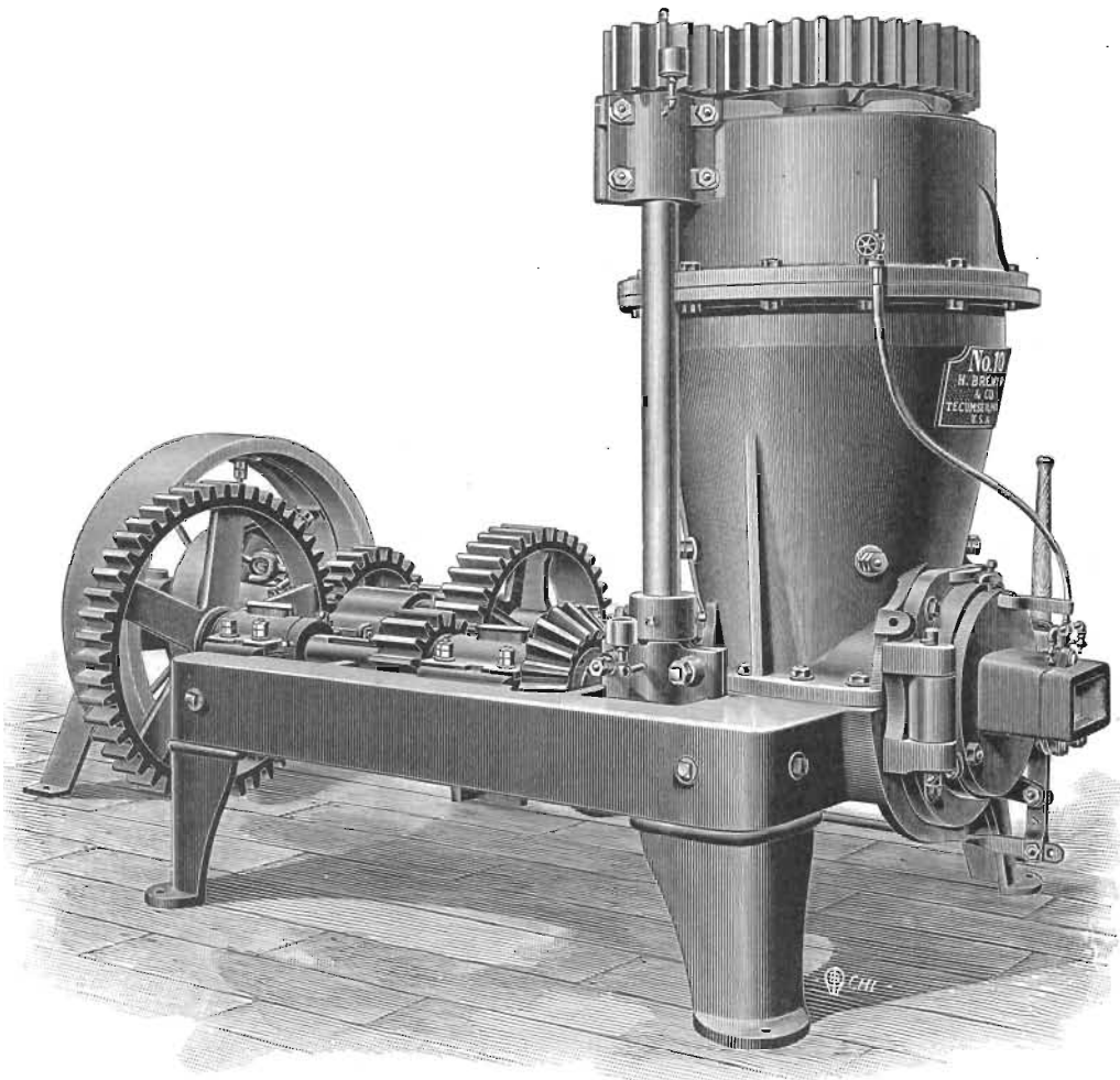
FIG. 19. Vertical Type of Stiff Mud Brick and Tile Machine.
