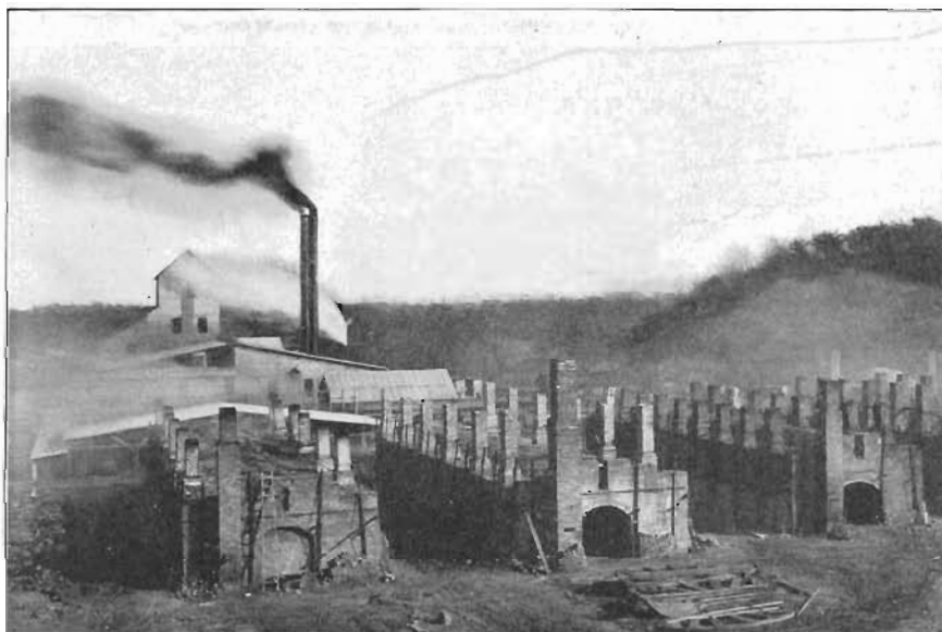
FIG. 53. A portion of the plant of the Iowa Brick Company showing multiple stack kilns in the foreground and the machinery buildings in the background.
