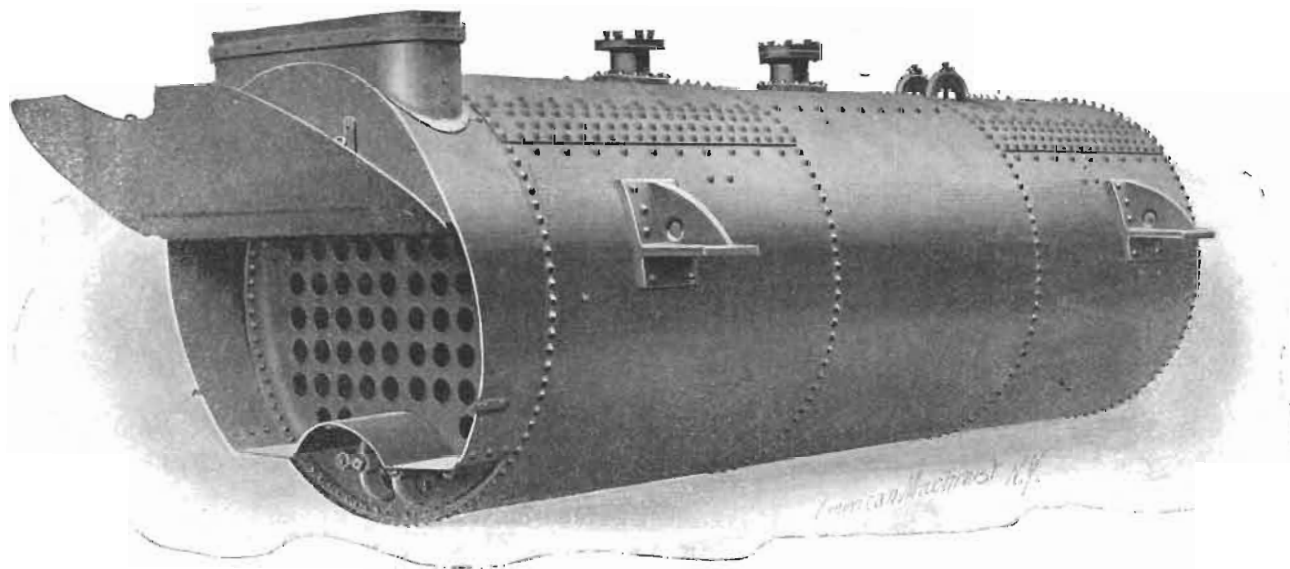
PLATE XI. Domeless boiler with nozzles, shell extended and fitted with flue door and up-take for half-arch front, manhole exposed, cast iron lugs; can be suspended.
