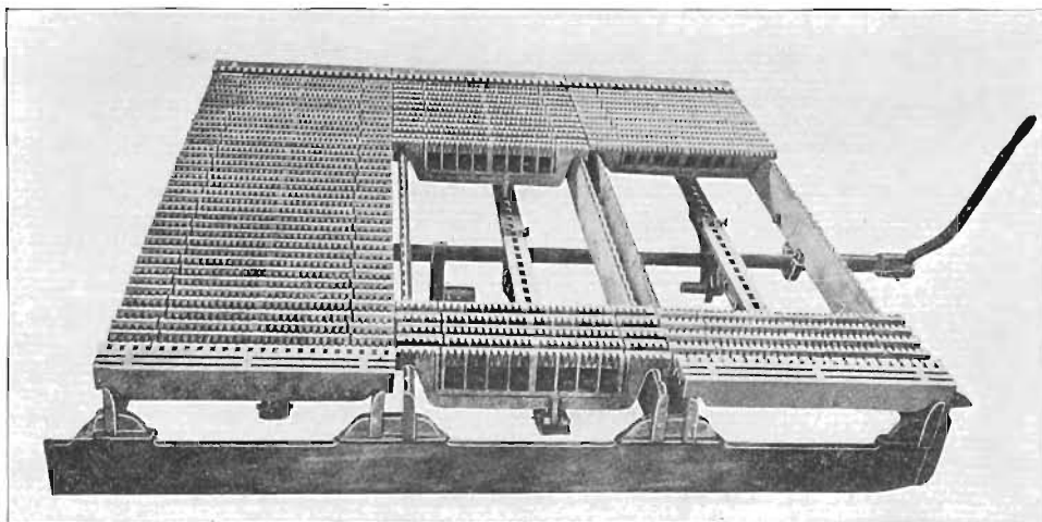
FIG. 93. A good type of rocking grate.
