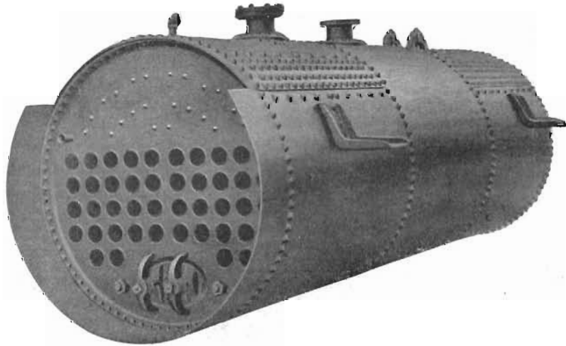
FIG. 32. Domeless boiler with nozzles, shell extended for full front, pressed steel lugs.
