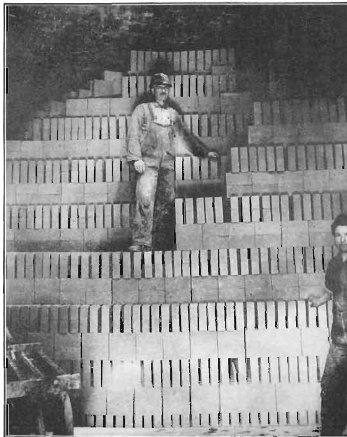
Method of facing dry press brick in a round, down draft kiln. Corey Pressed Brick and Coal Company, Lehigh, Iowa.
