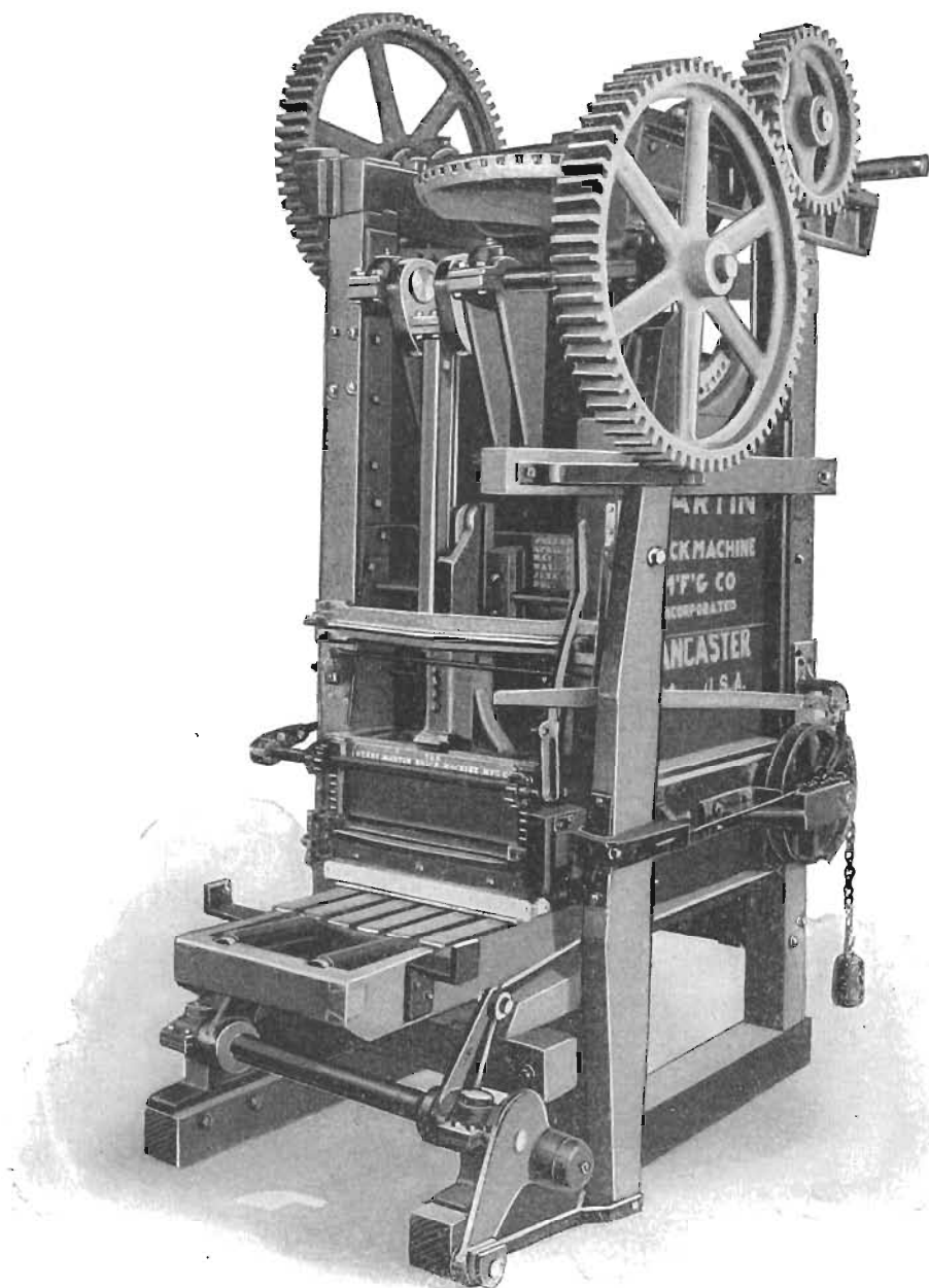
PLATE V. Vertical Type of Soft Mud Brick Machine
