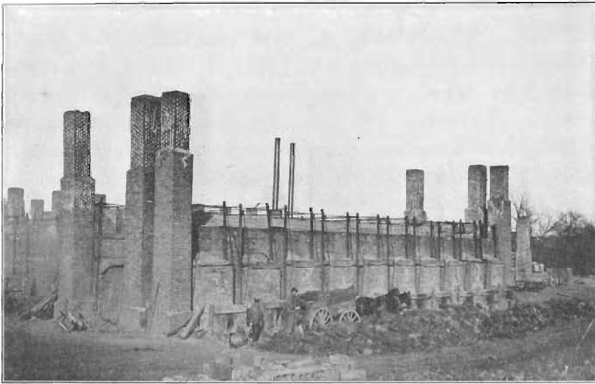
FIG. 29. Rectangular down draft kiln with stacks at the ends and showing ironing.
