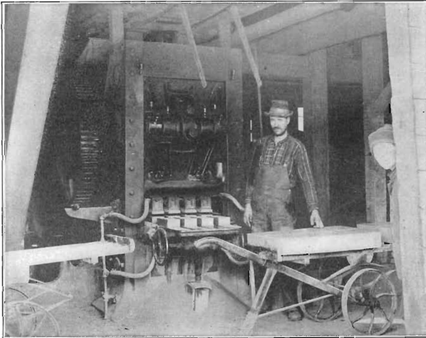
FIG. 66. Boyd four mold, dry press machine; Corey Pressed Brick and Coal Company, Lehigh, Iowa.
