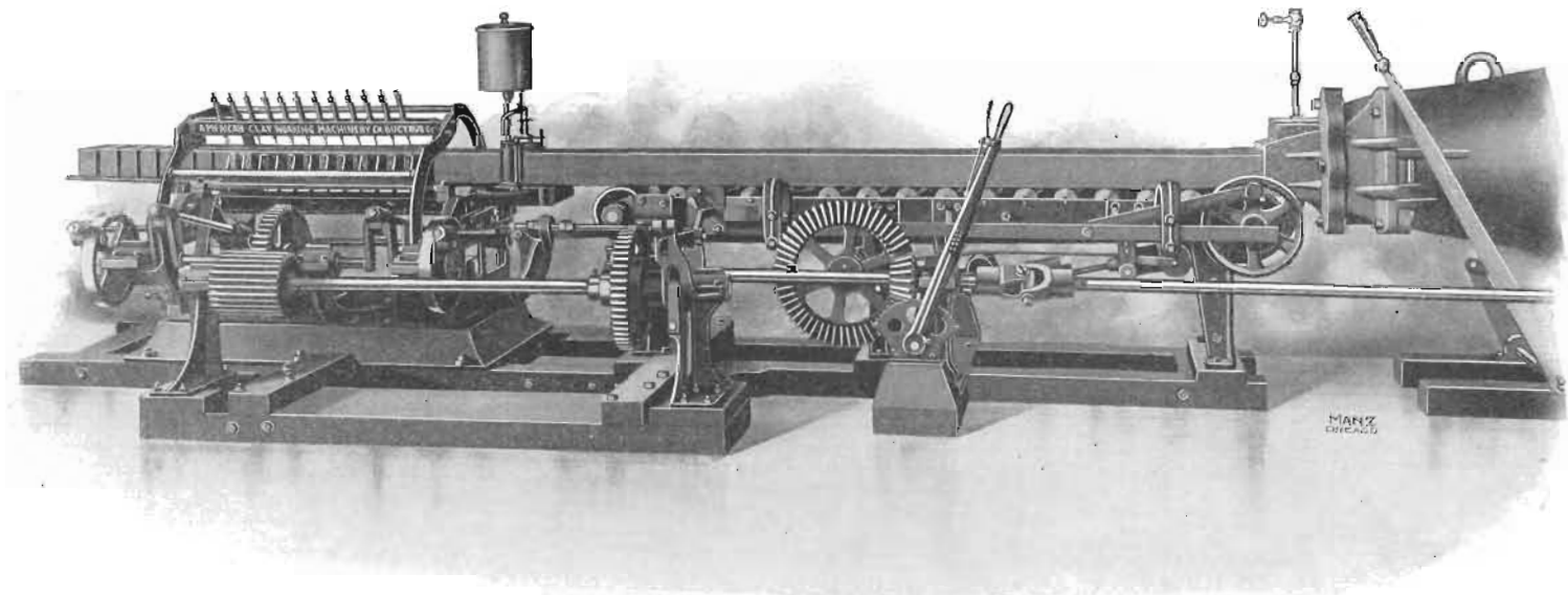
PLATE VIII. Automatic Oscillating Reciprocal Down Cut Table.
