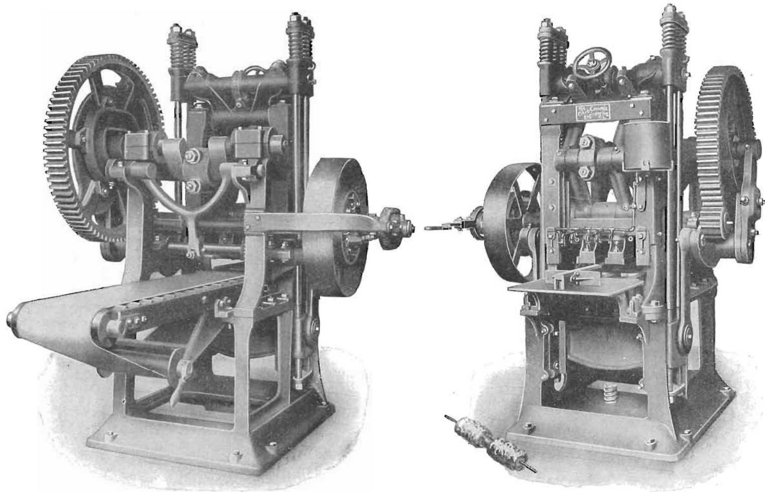
PLATE IX. The Richardson repress, front and back views.
