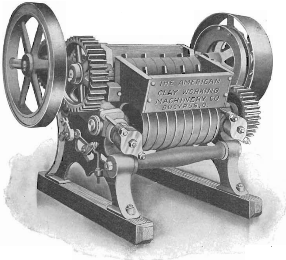
FIG. 9. Clay Crusher, Corrugated Rolls with Automatic Relief Feeder.
