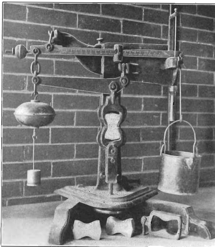
FIG. 1. Fairbanks machine used in measuring the tensile strength of clays.
