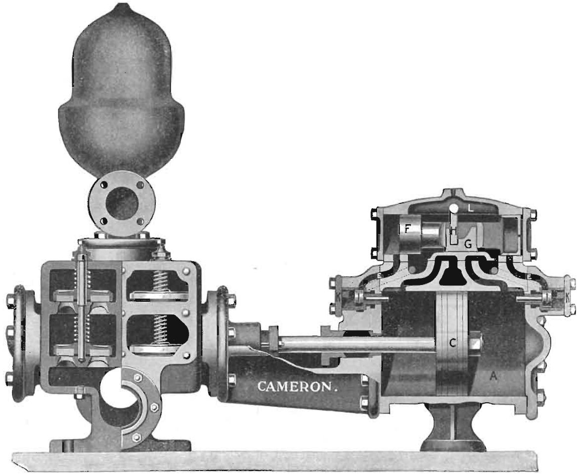
PLATE XV. Type of boiler feed-pump; simple, direct acting, in section.
