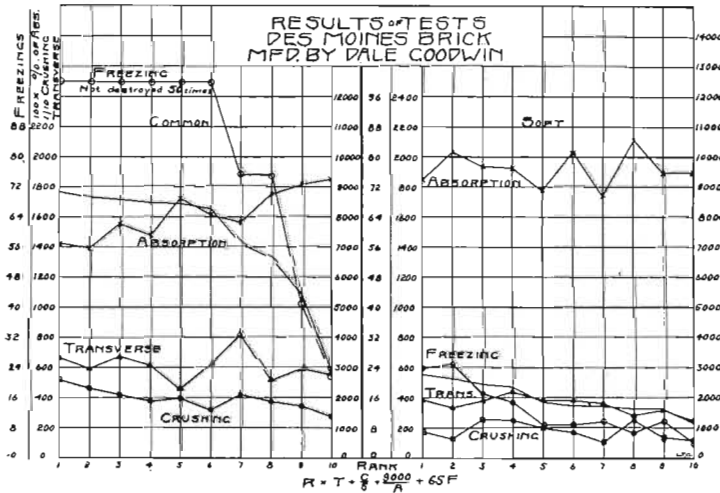
FIG. 103. Freezing tests, Goodwin brick.
