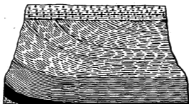
Figure 43. Clay at the Guthrie clay pit.
