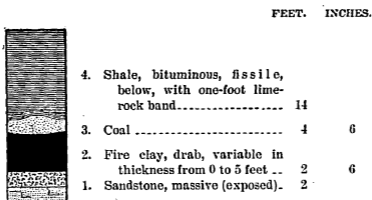
Figure 38. Coal bed in Williams mine, near New Sharon.
