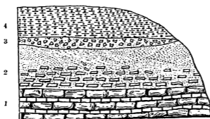
Figure 31. Quarry at Union Mills.
