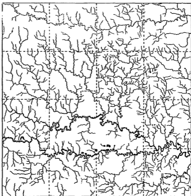
Figure 28. Sketch map showing the drainage of Keokuk county.
