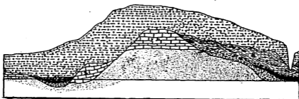
Figure 25. Diagrammatic section on Rock creek (west branch, Tp. 69 N., R. IX W., sec. 24, Nw. qr.), showing erosion unconformity between the Saint Louis and Des Moines formations.
