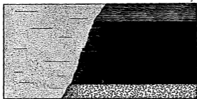
Figure 29. Cutout in What Cheer No. 5.
