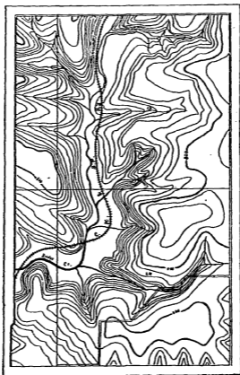
Figure 27. Topographic map of the region near Rowley's mine, north of Sigourney. Contours 10 feet; scale 2 inches to the mile.
