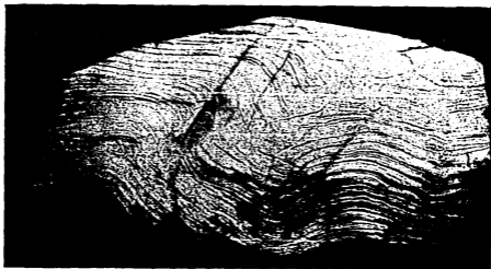
Figure 16. Contorted lamina in breccia fragment of second stage; from below Robins.
