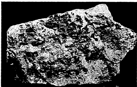
Figure 11. Dark flint and limestone from Fifth avenue sewer, Cedar Rapids.
