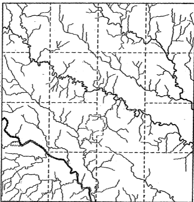
Figure 30. Drainage of Mahaska county.
