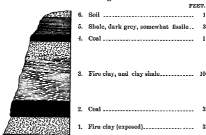
Figure 42. Bluff at Griffith drift; Given.
