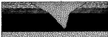
Figure 36. Drift channel in coal; Excelsior mine, Carbonado.
