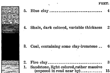
Figure 39. Seam of coal in Columbia shaft. Rose Hill.
