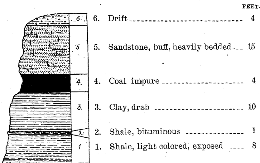
FIG. 51. Railroad cutting near east county line, below Runnells.
