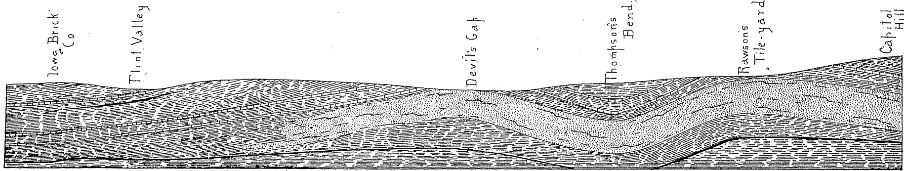
GEOLOGICAL SECTION FROM CAPITOL HILL TO THE MOUTH OF BEAVER CREEK.
