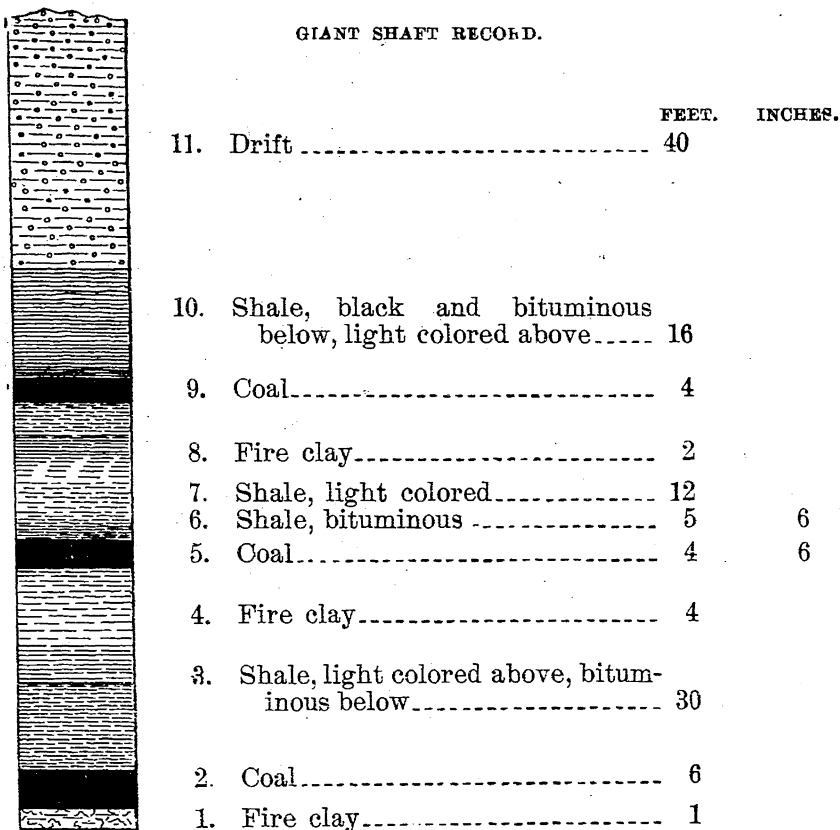
FIG. 51. Shaft of Giant No. 1. East Des Moines.
