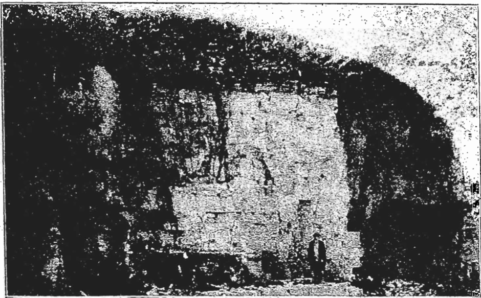
FIG. 2. View in the old McCune Quarry, Anamosa Limestone, Cedar Township, Johnson County, Iowa.
