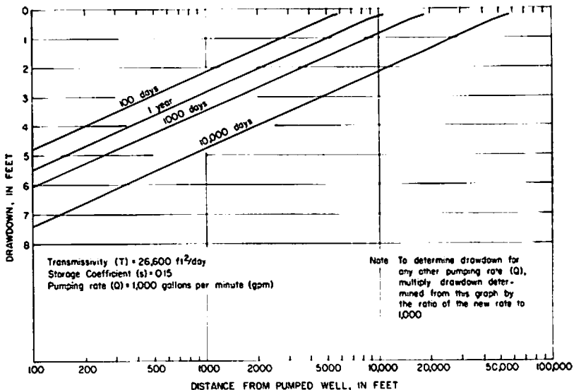
Figure 28.—Distance-drawdown graph.
